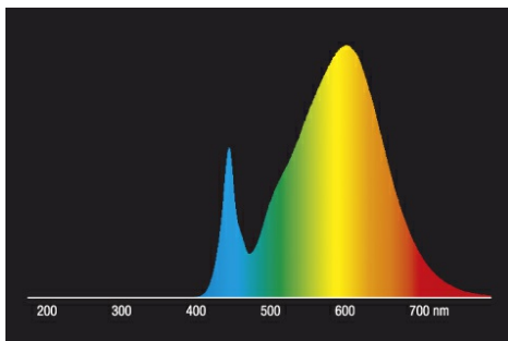
LED retrofit standard lamps 40W replacement, 2700K
