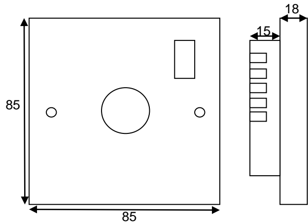
PIR0901S Switched Ceiling/wall Mounted PIR Movement Sensor
